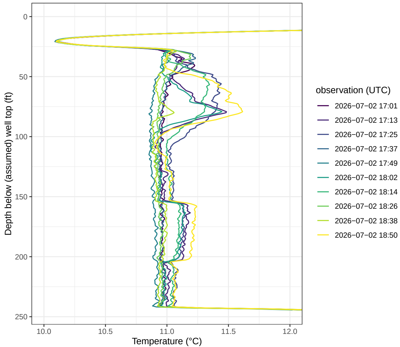
Darcy Observation Well – temperature vs depth
